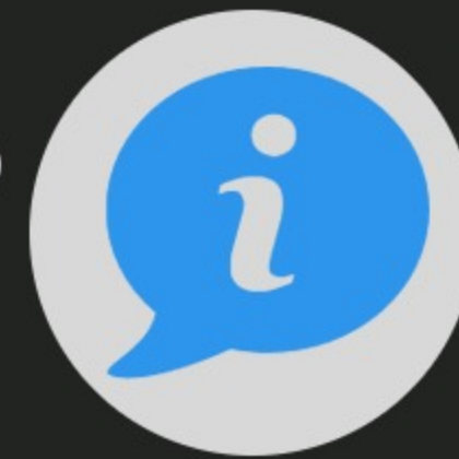
Informative
