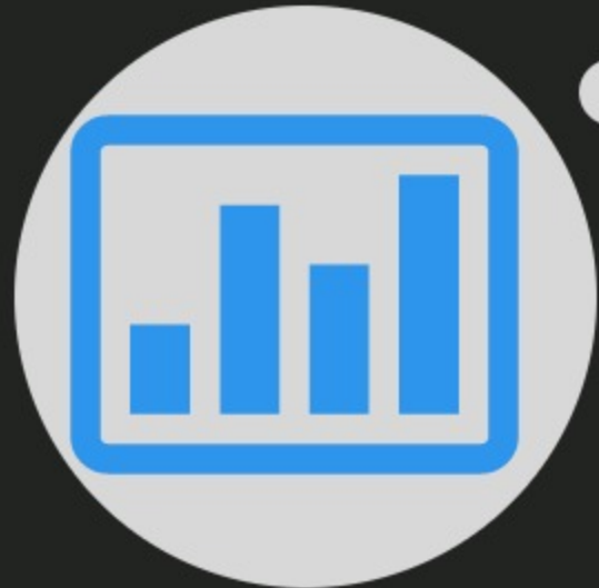
Statistical
