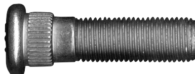
WS-404 Thread M12 - 1.50 Length 46mm
