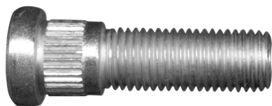
WS-312 Thread M12 - 1.50 Length 44.5mm
