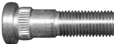
WS-336 Thread M12 - 1.25 Length 37.5mm
