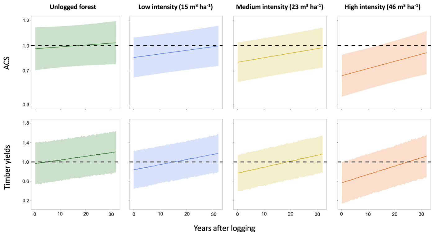
Fig. 2. Model predictions of recovery of ACS (a, b, and c) and timber stock (d, e, and f) at low, medium and high logging intensities. Observed ACS post-logging is weighted by initial ACS ( \text{Mg C ha}^{-1} ) and timber stock ( \text{m}^3 \text{ ha}^{-1} ). Solid lines are the mean predictions based on parameter and sampling uncertainty, with 95% credible intervals represented by the lighter colored ribbons. Predictions above the dashed horizontal line ( y -intercept = 1.0) indicate recovery to pre-logging values.
