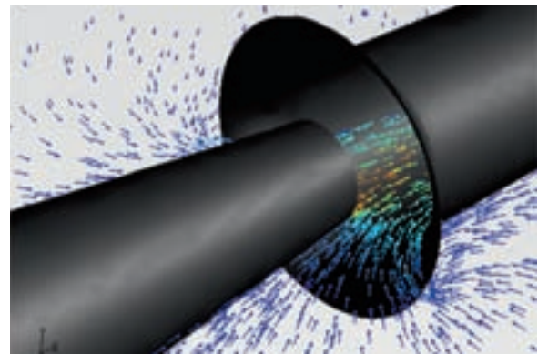
The computer fluid dynamic simulation shows the unique interaction between the discharge nozzle and the ejector pipe. The primary flow is enhanced by the subsequent generation of the secondary flow.
