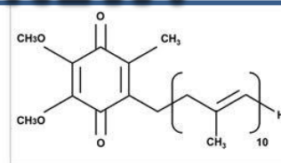
Structure of CoQ10
