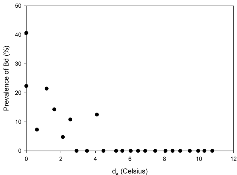
Figure 2. Prevalence of infection by Bd relative to d_e , the difference between temperatures in microhabitats used by frogs and the range of temperatures at which Bd grows best.
