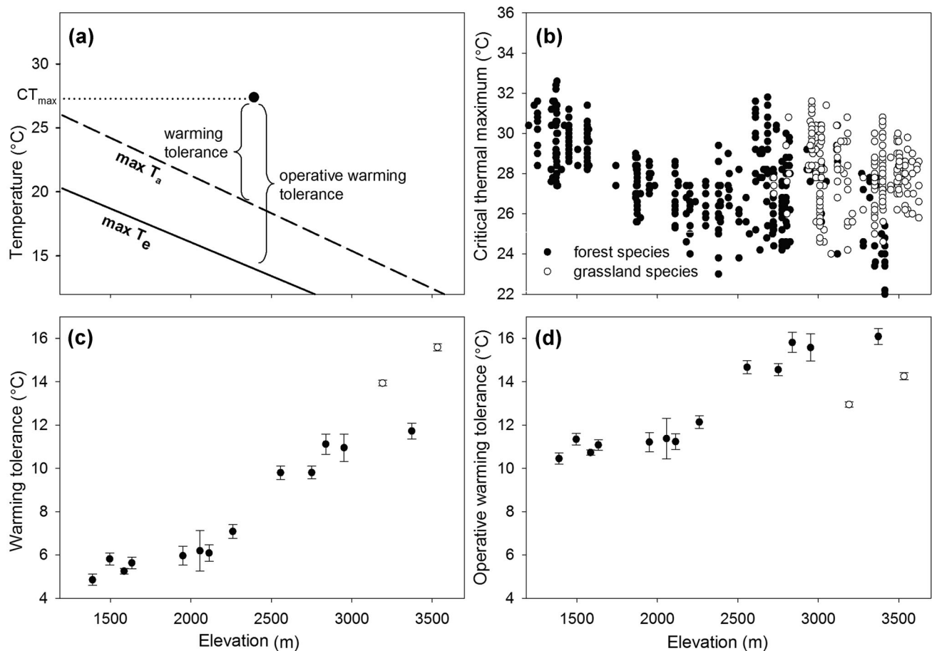
Figure 1. (a) Warming tolerance and operative warming tolerance as a function of average maximum temperature along the elevational gradient in the upper Kosñipata valley (Manu National Park, Peru) ( T_a , maximum air temperatures; T_e , maximum operative temperatures; CT_{max} , critical thermal maxima). (b) Critical thermal maxima for 383 forest (solid) and 254 grassland (open) strabomantid frogs ( n = 637 individuals of 15 species) along the elevational gradient. Average (SE) (c) warming tolerance and (d) operative warming tolerance of 15 species of strabomantid frogs.
