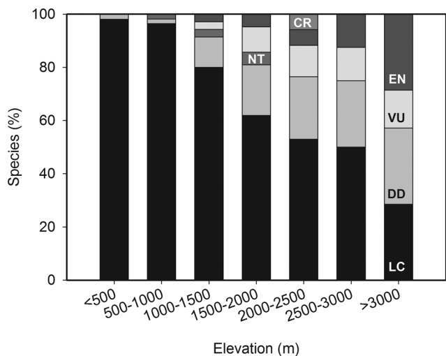
Figure 3. Proportion of amphibians considered threatened in Manu National Park, Peru (IUCN 2013) (Supporting Information) (LC, least concern; DD, data deficient; NT, near threatened; VU, vulnerable; EN, endangered; CR, critically endangered).
