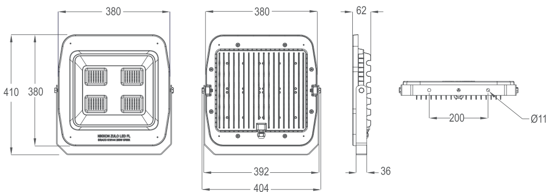
K10144 200W
