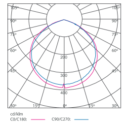
K10144 200W
