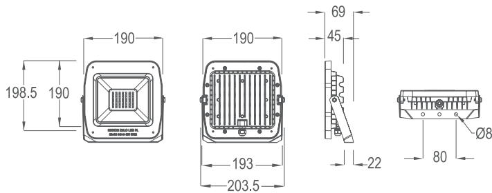
K10142 100W
