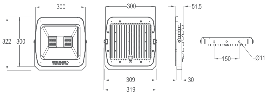
K10142 100W
