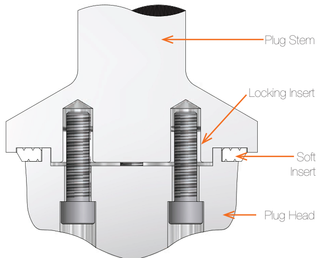
SOFT SEATED PLUG (FIGURE 7)
