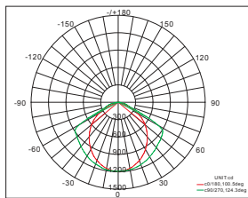
Luminous Intensity Distribution
