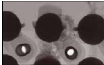
Minuscule solder dendrites and voids
